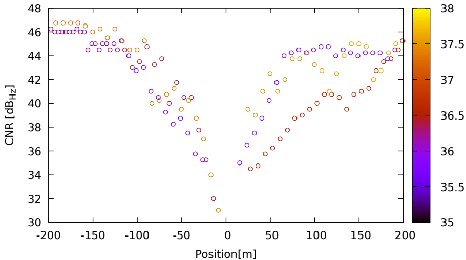
CNR vs position for R18 (G2) on LeicaGS18 - DOY 263 jam. 1
