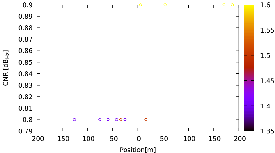
CNR vs position for 26 (G1) on SamsungS20 - DOY 263 jam. 2
