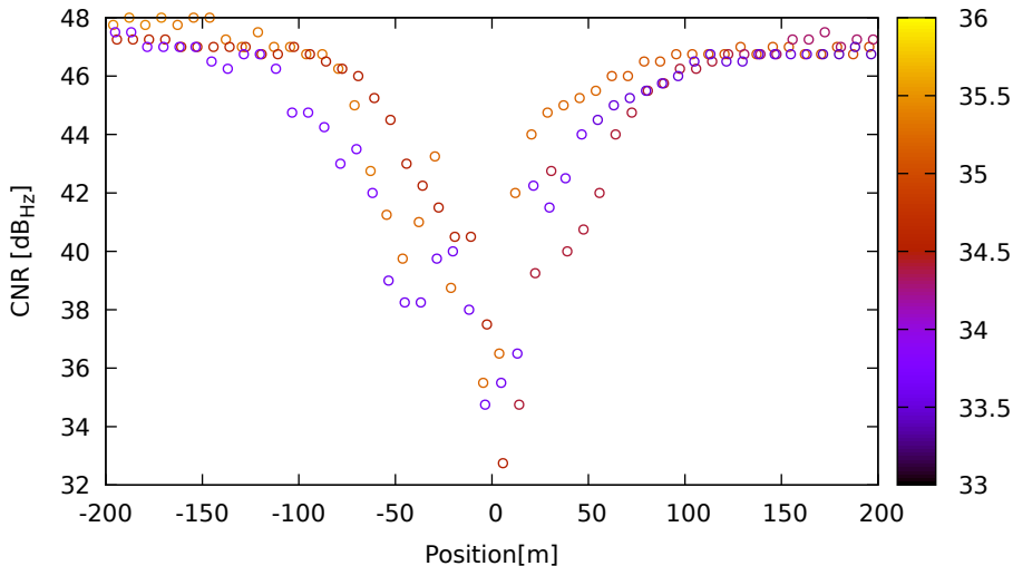
CNR vs position for C11 (B1) on SamsungS20 - DOY 263 jam. 1
