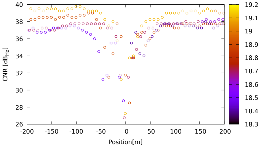
CNR vs position for C16 (B1) on SamsungS20 - DOY 263 jam. 2
