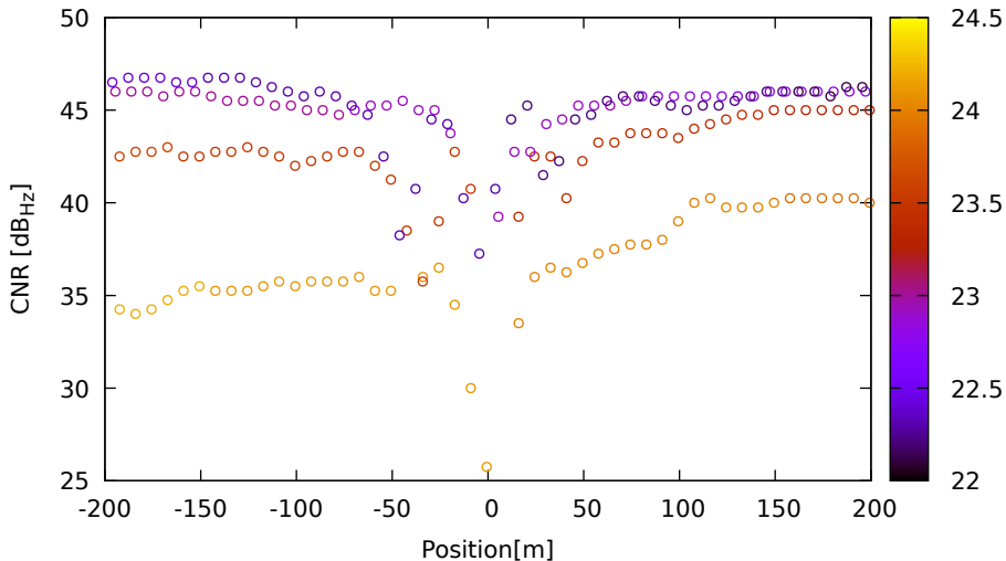
CNR vs position for C21 (B1) on SamsungS20 - DOY 263 jam. 2
