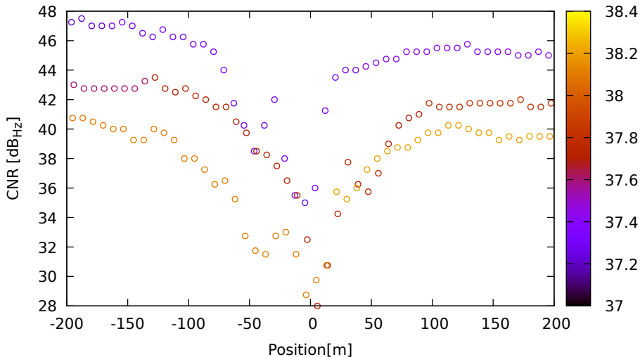
CNR vs position for C28 (B1) on SamsungS20 - DOY 263 jam. 1
