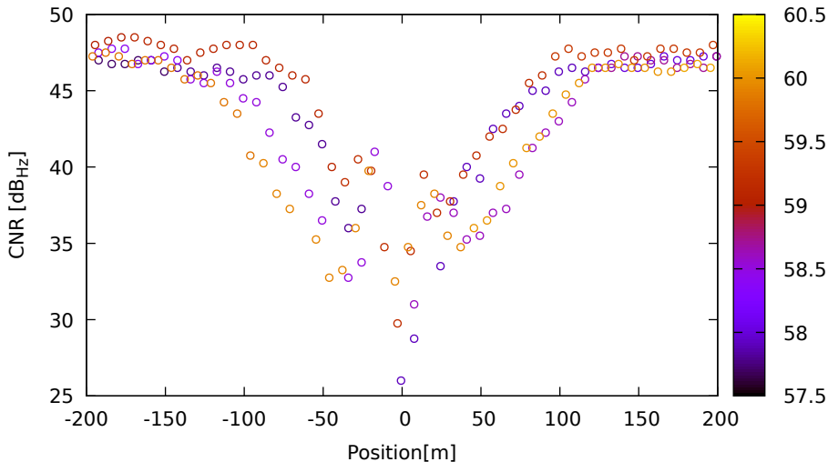
CNR vs position for E04 (E1) on SamsungS20 - DOY 263 jam. 2
