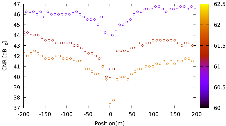
CNR vs position for E04 (E1) on SamsungS20 - DOY 263 jam. 3
