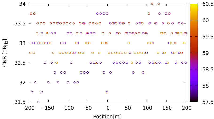
CNR vs position for E04 (E5a) on SamsungS20 - DOY 263 jam. 2
