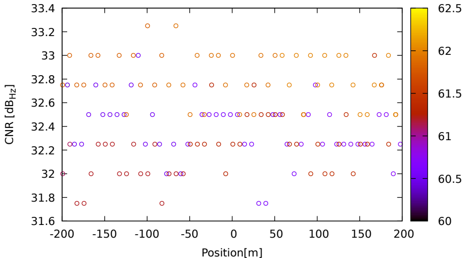
CNR vs position for E04 (E5a) on SamsungS20 - DOY 263 jam. 3
