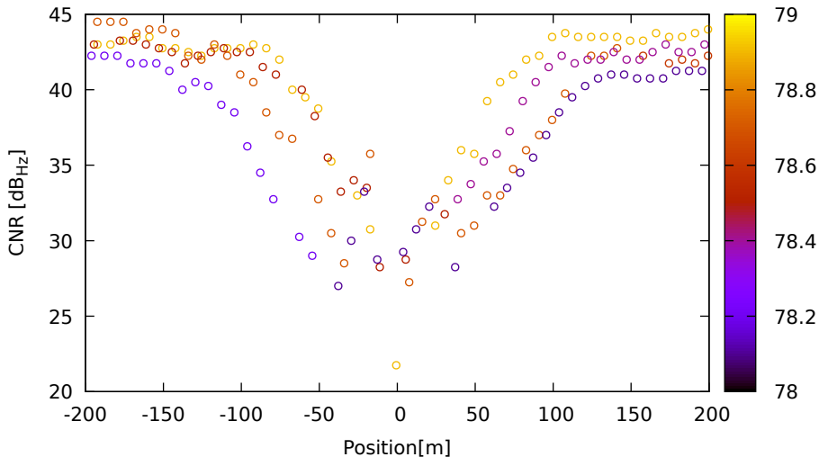
CNR vs position for E10 (E1) on SamsungS20 - DOY 263 jam. 2
