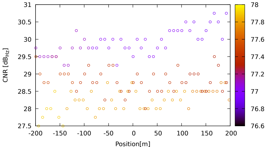
CNR vs position for E10 (E5a) on SamsungS20 - DOY 263 jam. 3
