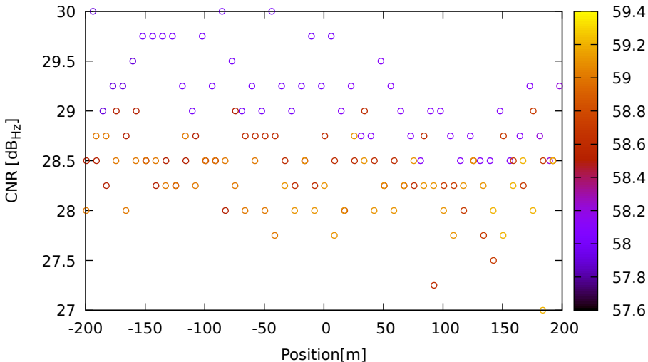
CNR vs position for E11 (E5a) on SamsungS20 - DOY 263 jam. 3
