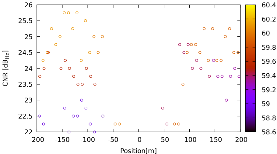
CNR vs position for E19 (E5a) on SamsungS20 - DOY 263 jam. 1
