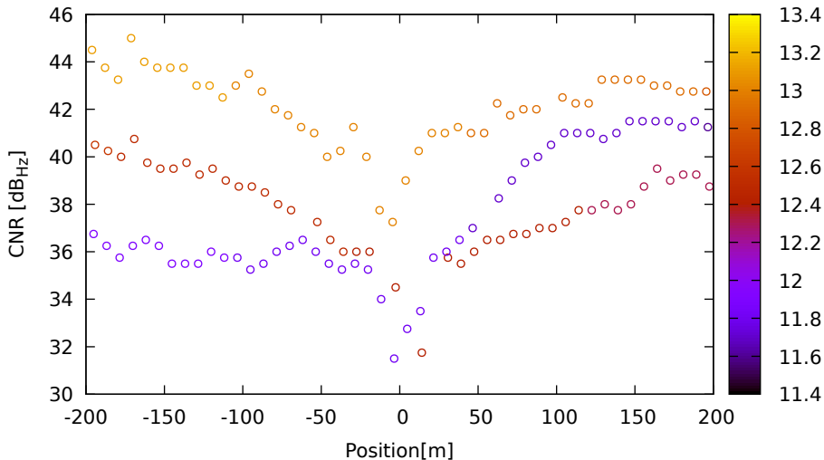
CNR vs position for E33 (E1) on SamsungS20 - DOY 263 jam. 1
