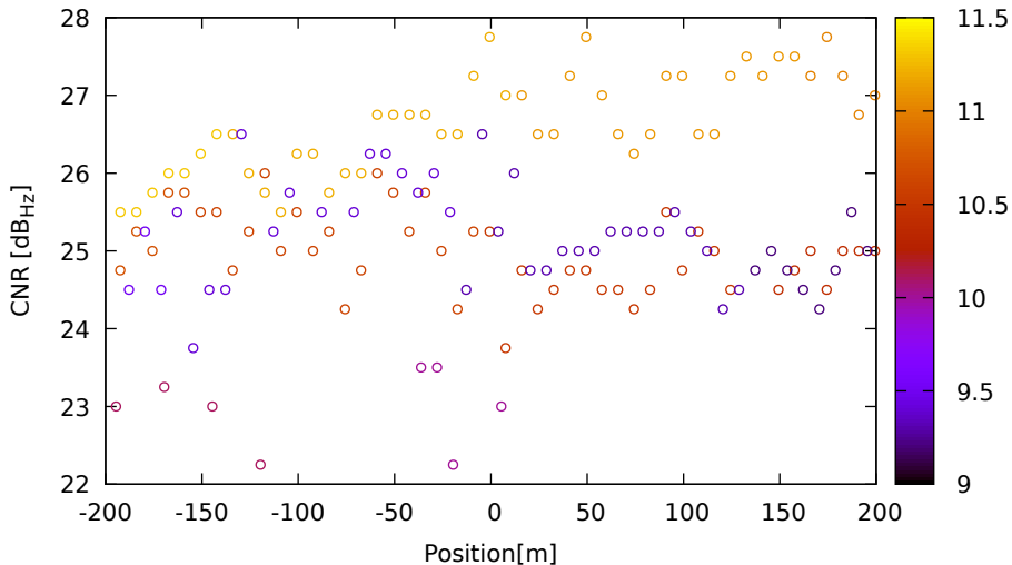
CNR vs position for E33 (E5a) on SamsungS20 - DOY 263 jam. 2
