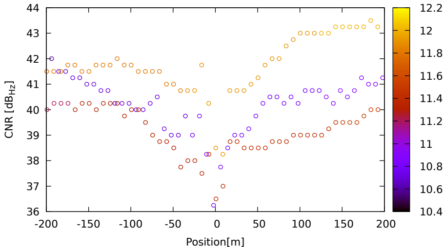
CNR vs position for E36 (E1) on SamsungS20 - DOY 263 jam. 3
