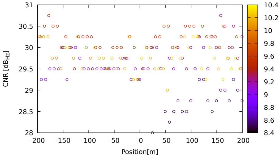
CNR vs position for E36 (E5a) on SamsungS20 - DOY 263 jam. 2
