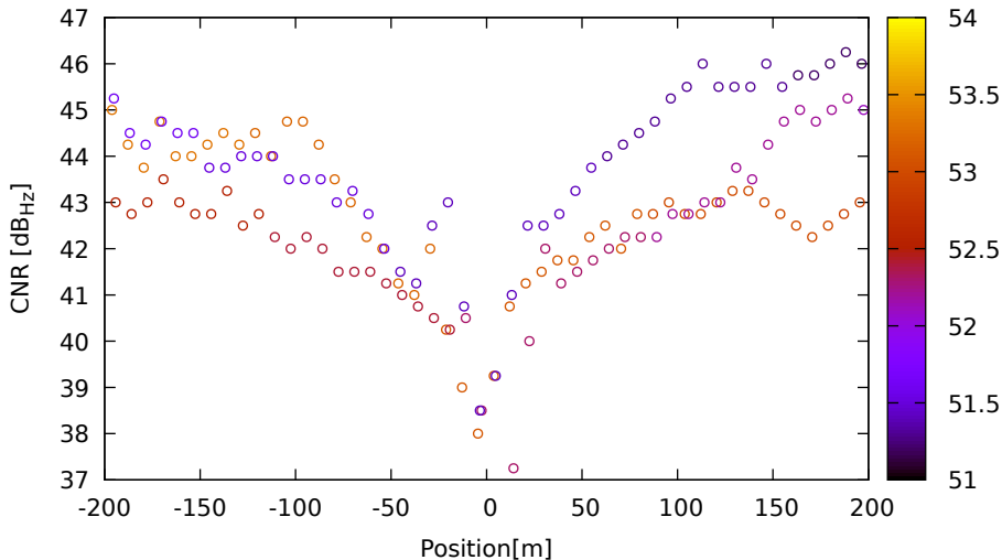
CNR vs position for G01 (L1) on SamsungS20 - DOY 263 jam. 1
