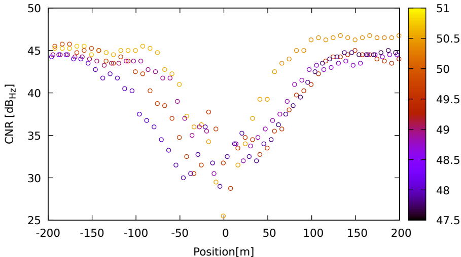
CNR vs position for G01 (L1) on SamsungS20 - DOY 263 jam. 2
