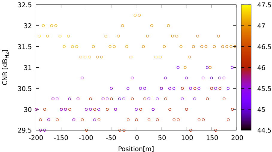
CNR vs position for G01 (L5) on SamsungS20 - DOY 263 jam. 3
