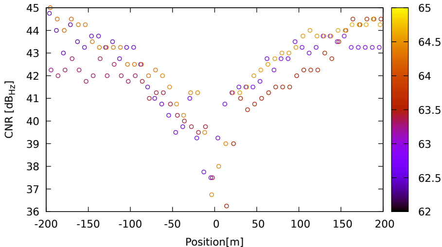
CNR vs position for G04 (L1) on SamsungS20 - DOY 263 jam. 1
