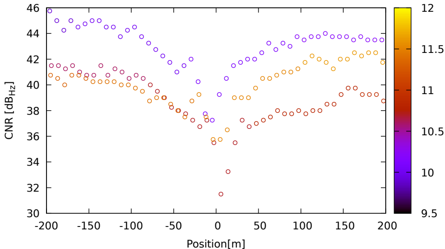
CNR vs position for G06 (L1) on SamsungS20 - DOY 263 jam. 1
