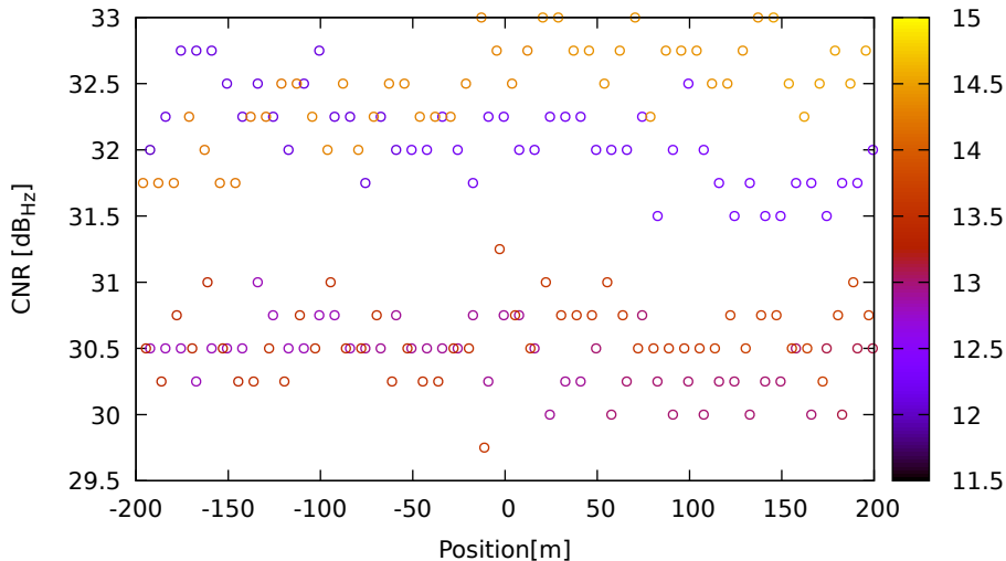
CNR vs position for G06 (L5) on SamsungS20 - DOY 263 jam. 2
