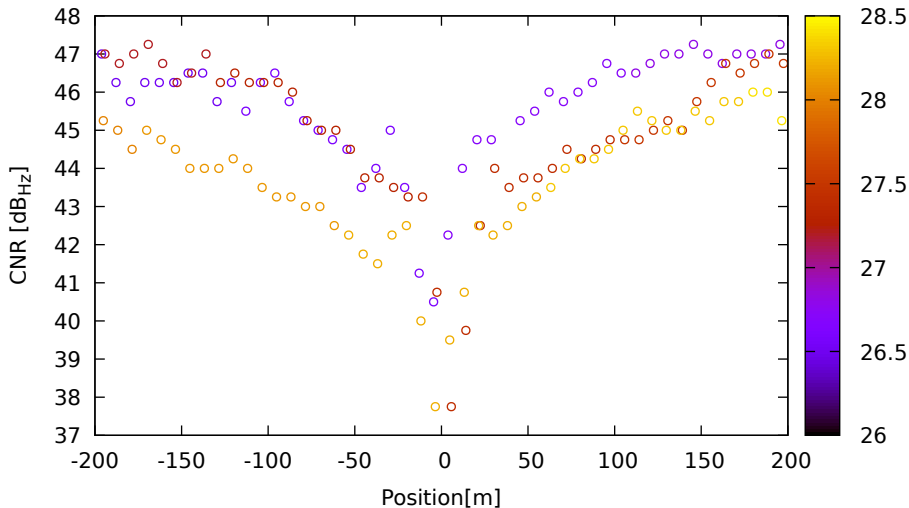
CNR vs position for G09 (L1) on SamsungS20 - DOY 263 jam. 1
