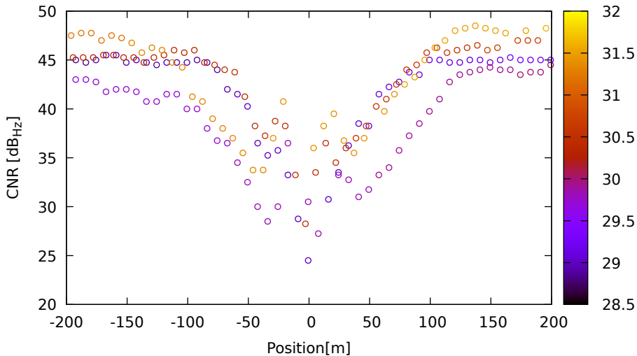
CNR vs position for G09 (L1) on SamsungS20 - DOY 263 jam. 2
