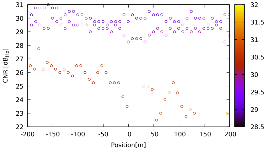
CNR vs position for G09 (L5) on SamsungS20 - DOY 263 jam. 2
