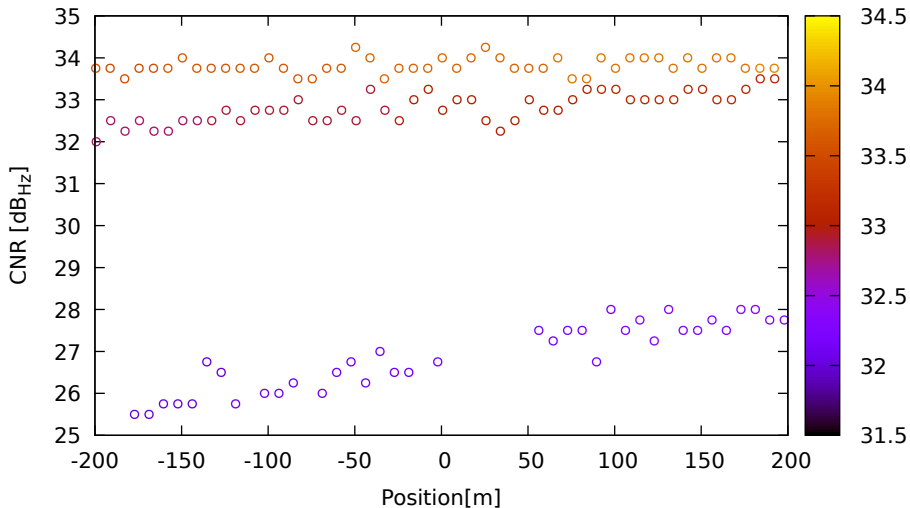
CNR vs position for G09 (L5) on SamsungS20 - DOY 263 jam. 3
