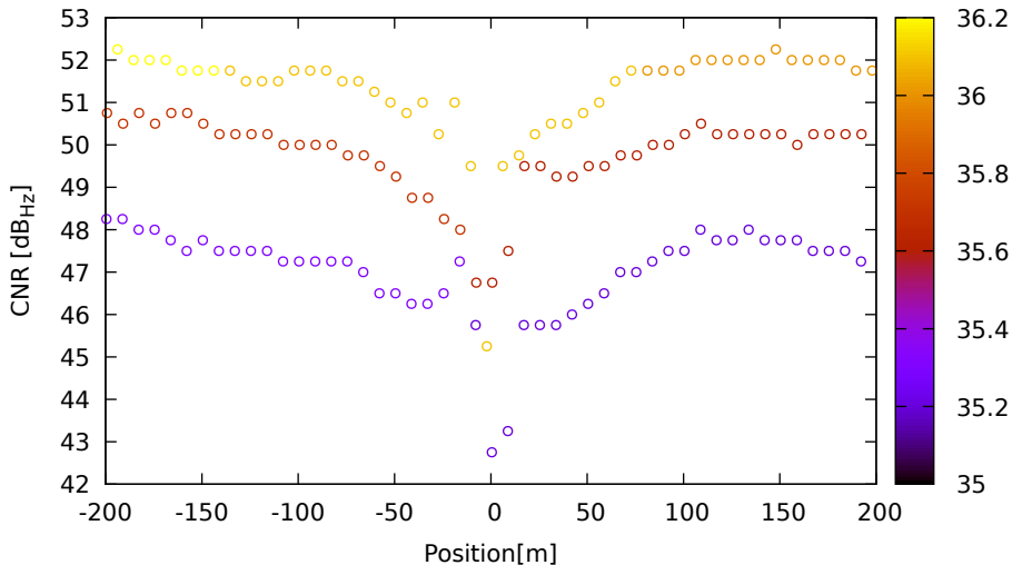
CNR vs position for G17 (L1) on SamsungS20 - DOY 263 jam. 3
