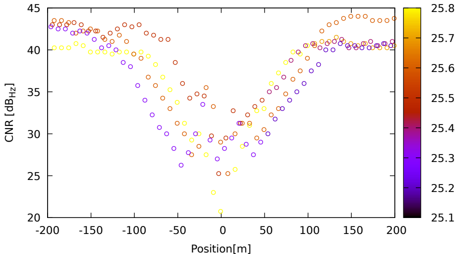
CNR vs position for G31 (L1) on SamsungS20 - DOY 263 jam. 2
