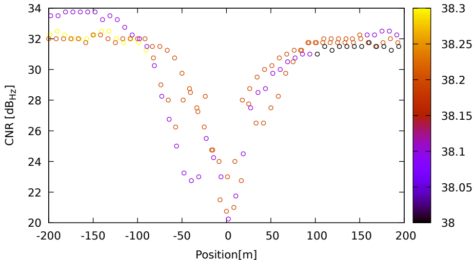
CNR vs position for C09 (B1) on Xiaomi11T - DOY 263 jam. 1
