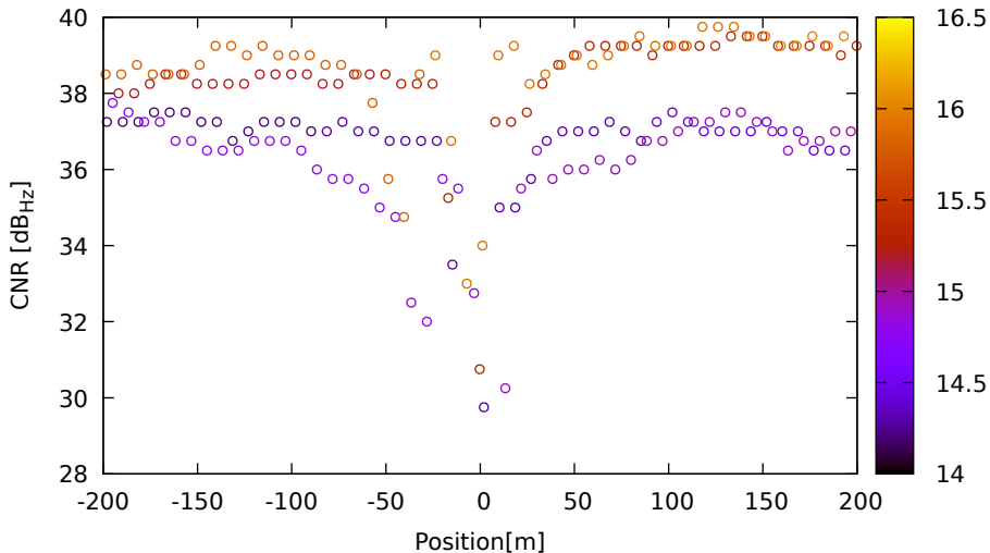
CNR vs position for C26 (B1) on Xiaomi11T - DOY 263 jam. 2
