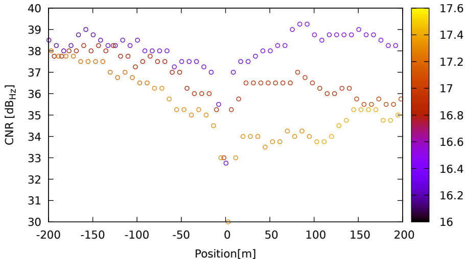
CNR vs position for C26 (B1) on Xiaomi11T - DOY 263 jam. 3
