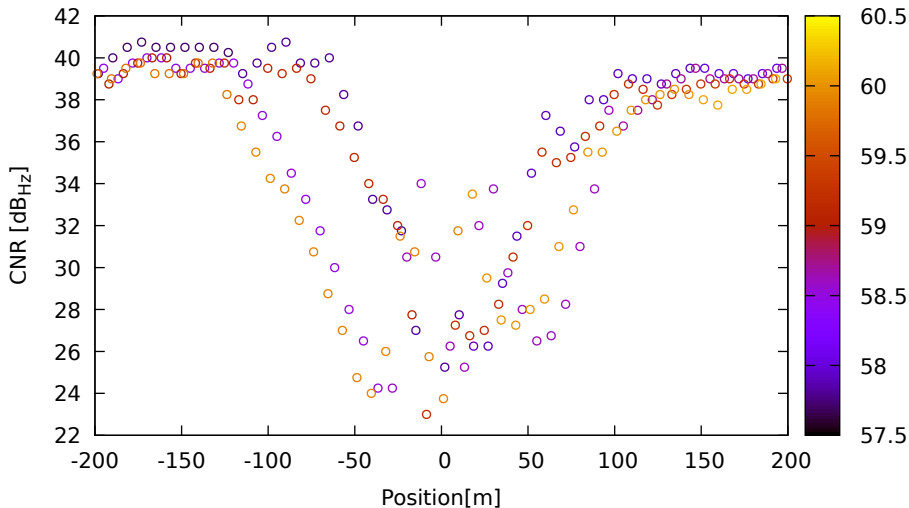
CNR vs position for E04 (E1) on Xiaomi11T - DOY 263 jam. 2
