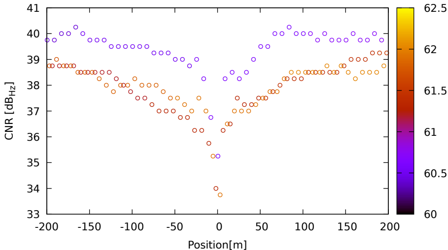
CNR vs position for E04 (E1) on Xiaomi11T - DOY 263 jam. 3
