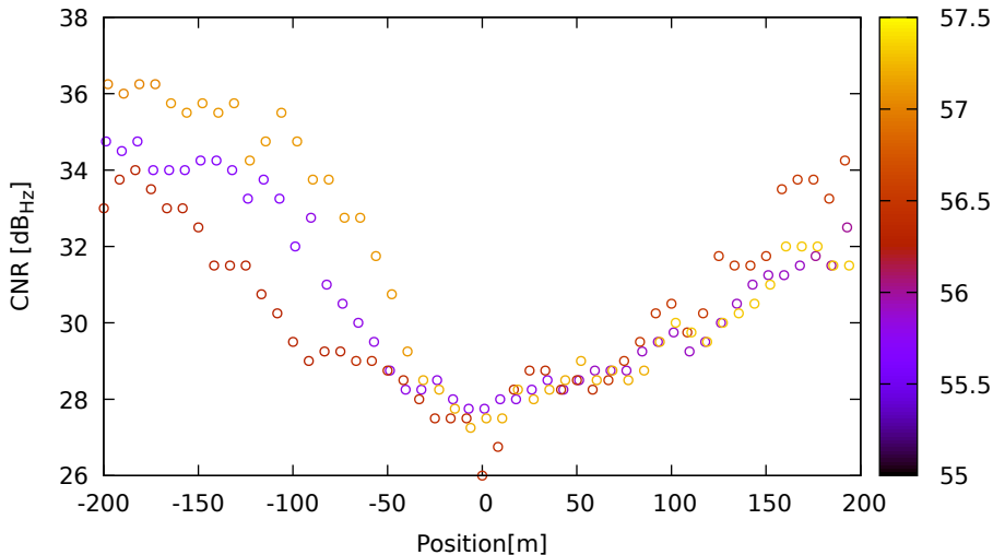
CNR vs position for E04 (E5a) on Xiaomi11T - DOY 263 jam. 1
