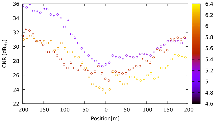
CNR vs position for E09 (E5a) on Xiaomi11T - DOY 263 jam. 1
