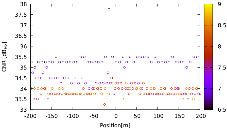
CNR vs position for E09 (E5a) on Xiaomi11T - DOY 263 jam. 2
