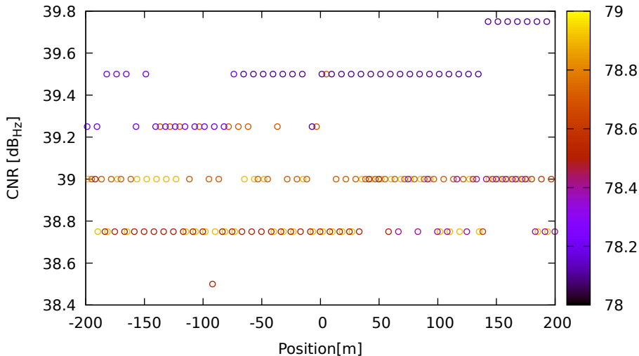
CNR vs position for E10 (E5a) on Xiaomi11T - DOY 263 jam. 2
