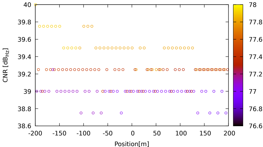
CNR vs position for E10 (E5a) on Xiaomi11T - DOY 263 jam. 3
