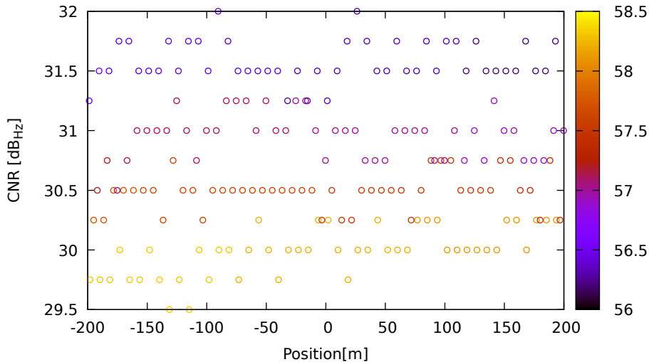
CNR vs position for E19 (E5a) on Xiaomi11T - DOY 263 jam. 2
