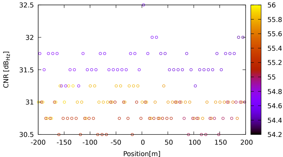
CNR vs position for E19 (E5a) on Xiaomi11T - DOY 263 jam. 3
