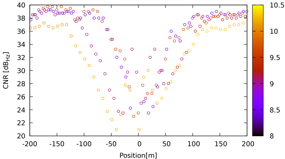
CNR vs position for E36 (E1) on Xiaomi11T - DOY 263 jam. 2
