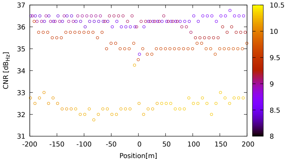
CNR vs position for E36 (E5a) on Xiaomi11T - DOY 263 jam. 2
