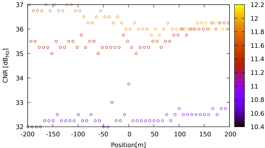
CNR vs position for E36 (E5a) on Xiaomi11T - DOY 263 jam. 3
