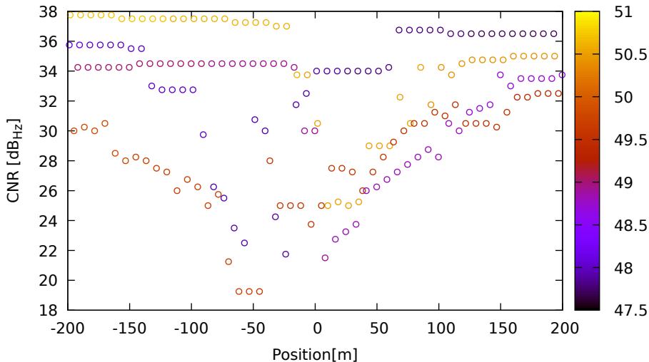
CNR vs position for G01 (L1) on Xiaomi11T - DOY 263 jam. 2
