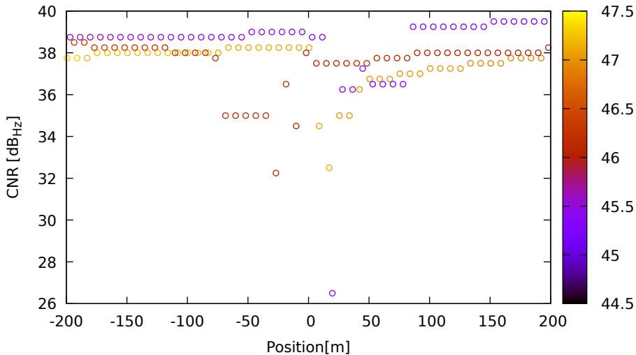
CNR vs position for G01 (L1) on Xiaomi11T - DOY 263 jam. 3
