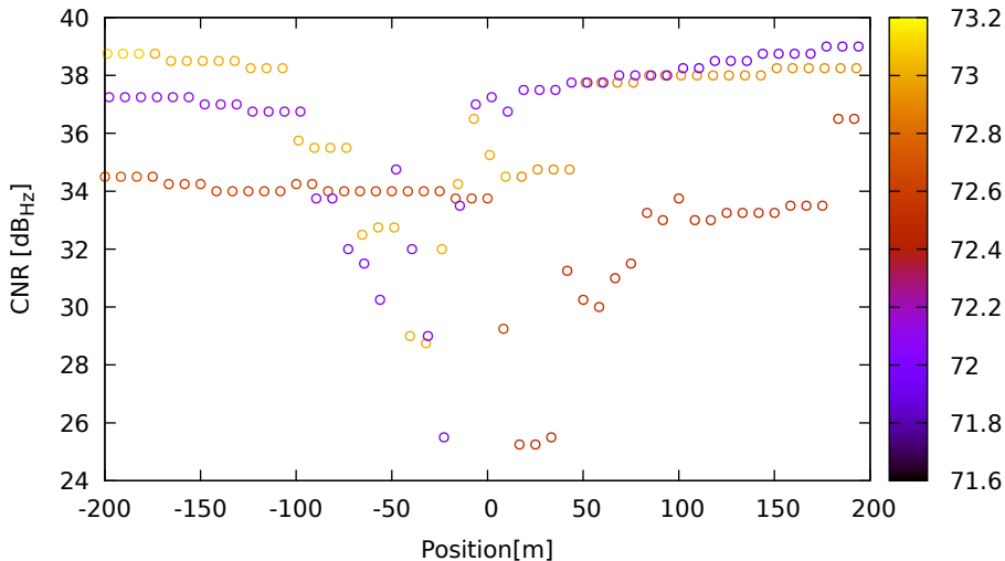
CNR vs position for G03 (L1) on Xiaomi11T - DOY 263 jam. 1
