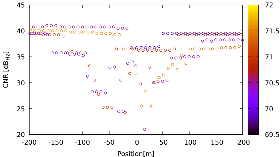
CNR vs position for G03 (L1) on Xiaomi11T - DOY 263 jam. 2
