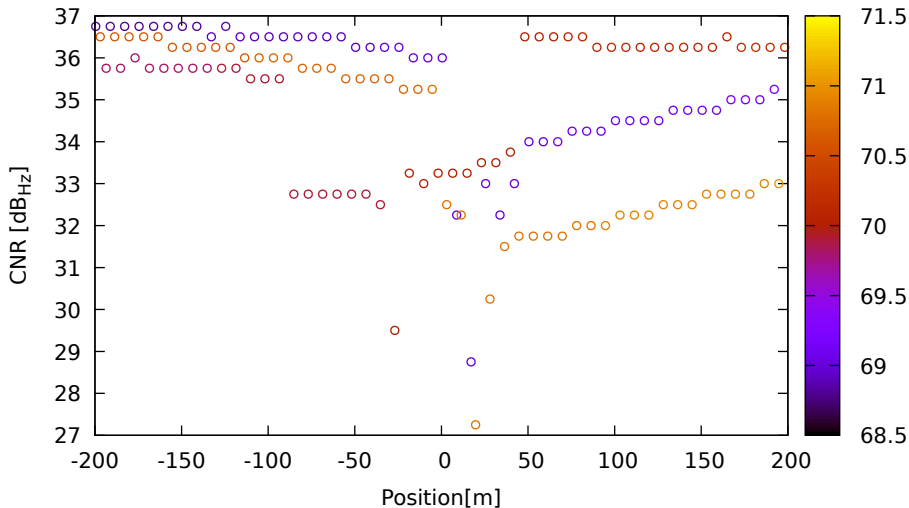
CNR vs position for G04 (L1) on Xiaomi11T - DOY 263 jam. 3
